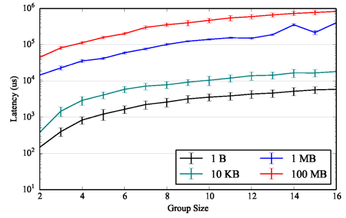
(b) Atomic multicast latency (TCP)
