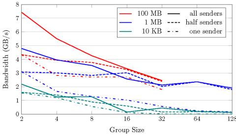
Fig. 14. Totally ordered (atomic multicast) mode.
